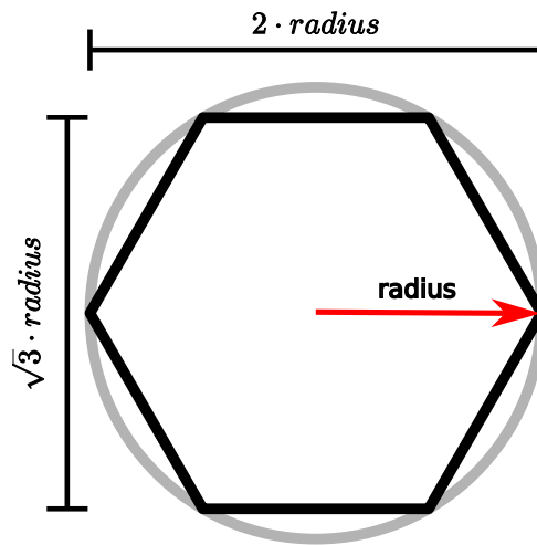
Figure 385: The size of an hexagon, calculated
